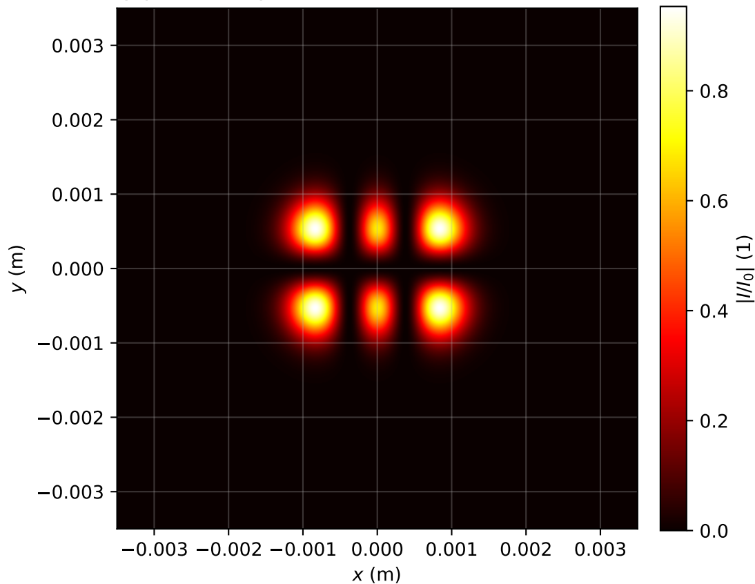
Intensity profile I(x, y, z = 0.716)/I_0 , P_{in}=0.5P_{cr} , artificial time
